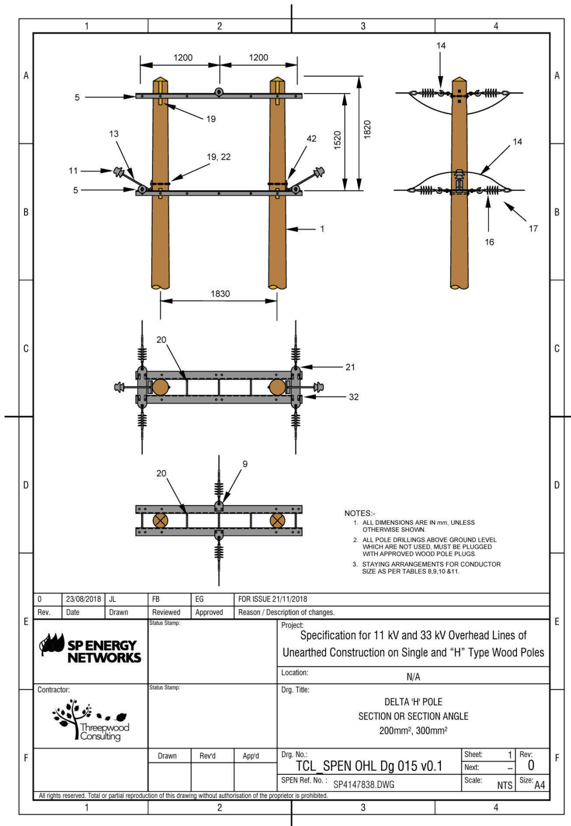
22.15 Figure 15 General Arrangement Delta "H" Pole Section or Section Angle 200mm 2 , 300mm 2 (Drawing No. SP4147838)
